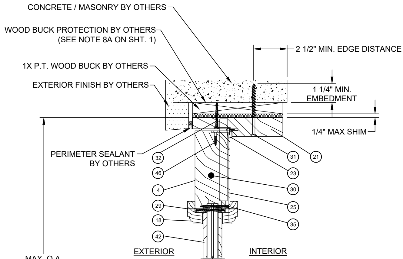
D VERTICAL SECTION OPAQUE DOOR AT HEAD CONCRETE / MASONRY SUBSTRATE
