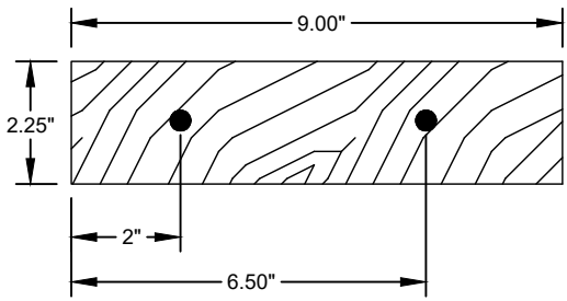
③ BOTTOM RAIL - GLAZED DOOR WOOD (0.44 MIN. S.G.)
