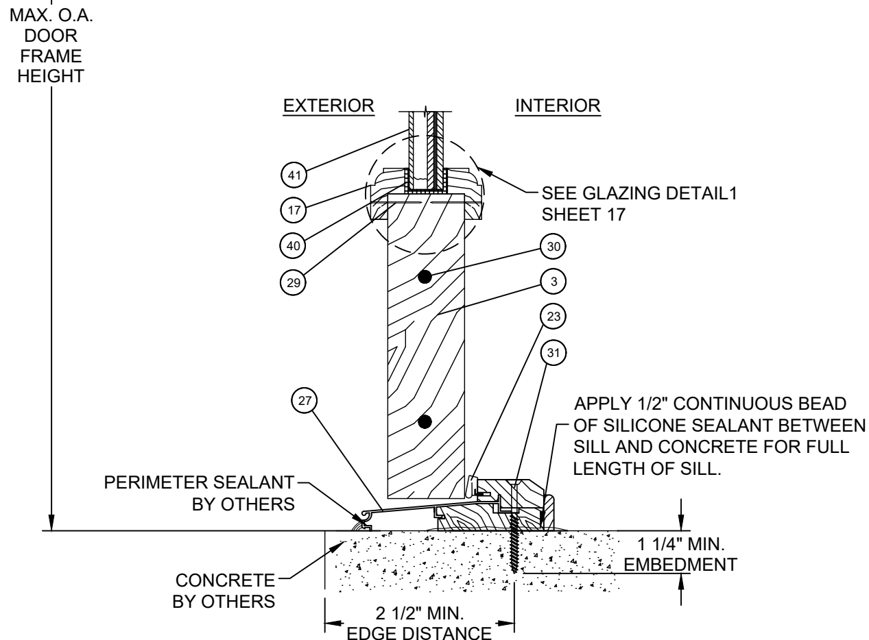
C VERTICAL SECTION GLAZED DOOR PANEL AT SILL CONCRETE / MASONRY SUBSTRATE
