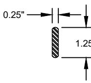
㉒ 1/4" X 1 1/4" REINFORCEMENT STEEL ASTM A1008 OR ASTM A366
