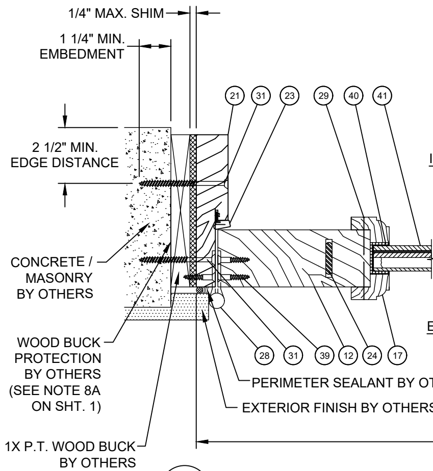
M HORIZONTAL SECTION CONCRETE / MASONRY SUBSTRATE GLAZED HINGE JAMB
