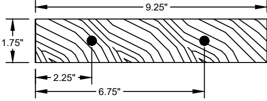
⑦ BOTTOM RAIL - GLAZED SIDELITE WOOD (0.44 MIN. S.G.)
