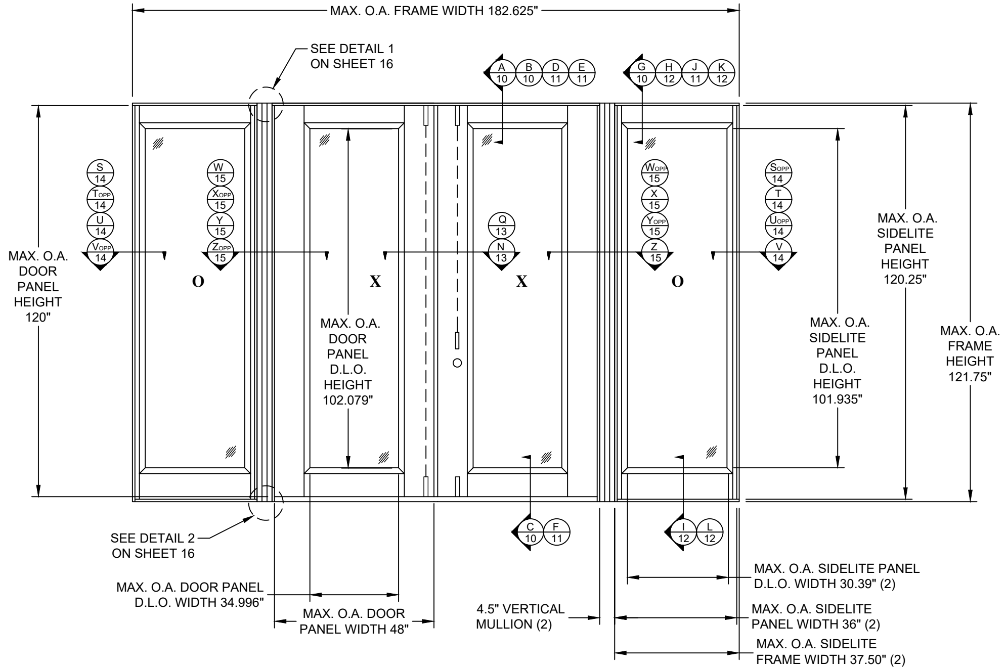
ELEVATION DOUBLE DOOR W / SIDELITES (OXXO) EXTERIOR VIEW
