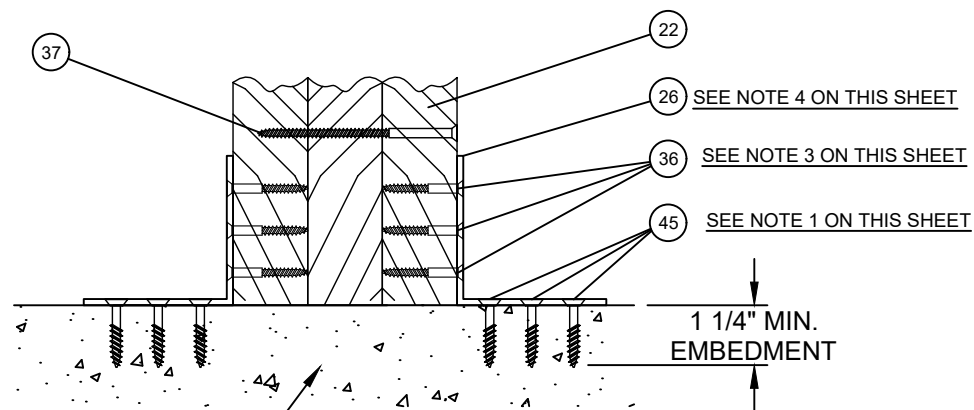
DETAIL 2 CONCRETE/ MASONRY & HEAD
