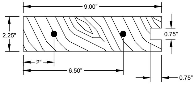
⑤ BOTTOM RAIL - OPAQUE DOOR WOOD (0.44 MIN. S.G.)
