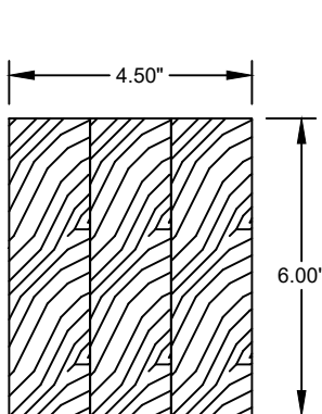
⑳ 4.5" VERTICAL MULLION (WOOD 0.44 MIN. S.G.)
