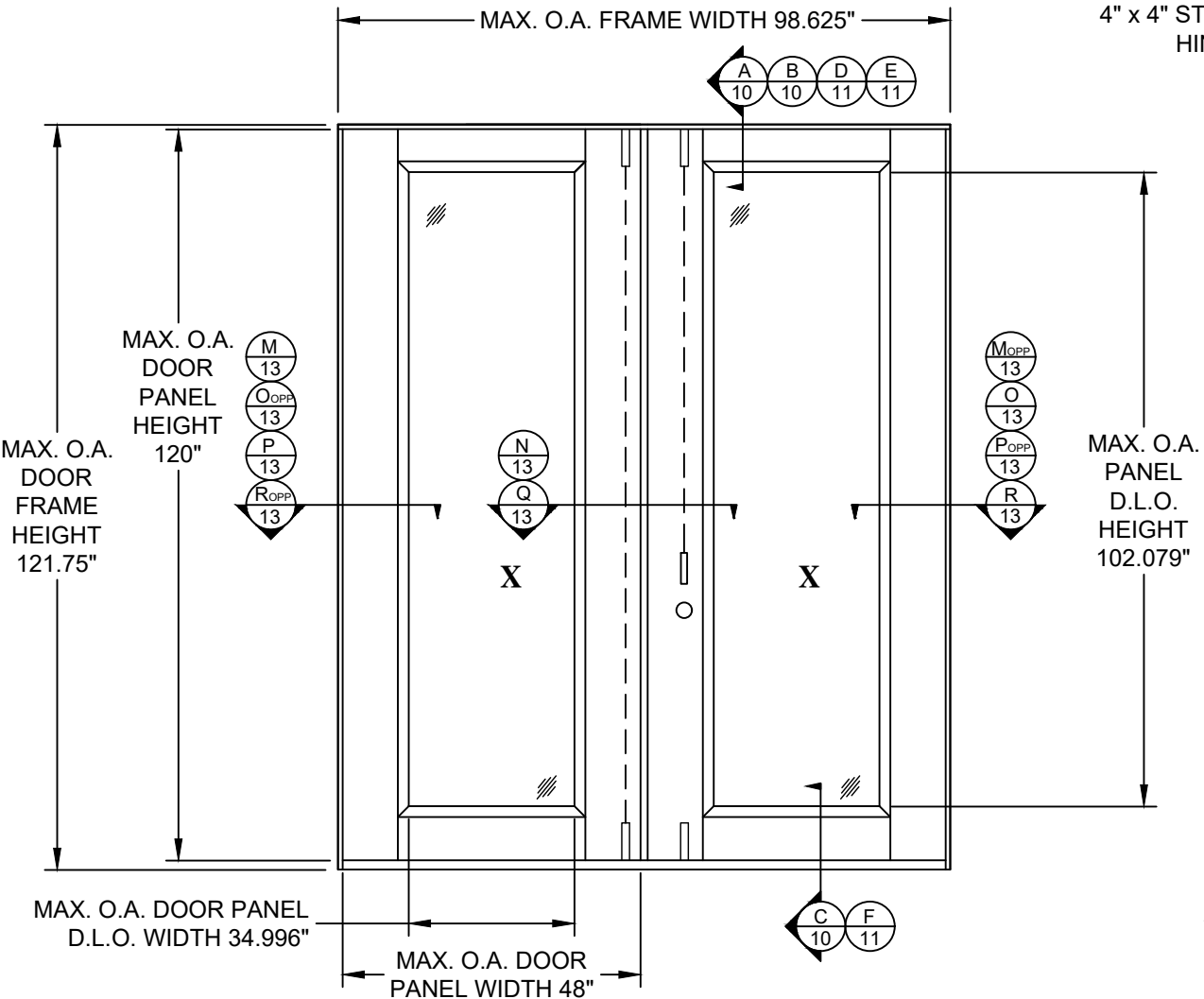
ELEVATION DOUBLE DOOR (XX) SQUARE TOP EXTERIOR VIEW
