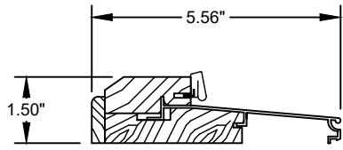
㉕ OUTSWING THRESHOLD 6063-T5 ALUMINUM / WOOD
