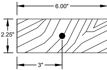
② TOP RAIL - GLAZED DOOR WOOD (0.44 MIN. S.G.)
