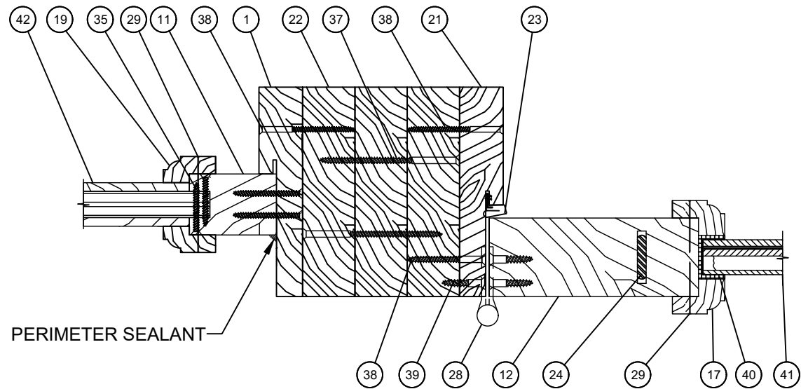
W HORIZONTAL SECTION MULLION OPAQUE SIDELITE / GLAZED DOOR PANEL
