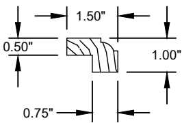
㉓ GLAZING BEAD - GLAZED DOOR WOOD (0.44 MIN. S.G.)
