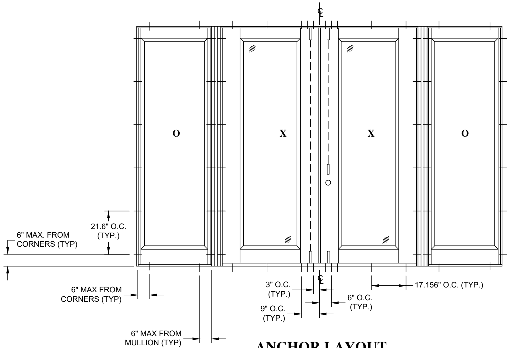
ANCHOR LAYOUT DOUBLE DOOR W / SIDELITES (OXXO) EXTERIOR VIEW
