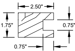
⑯ GLAZING BEAD - SIDELITE WOOD (0.44 MIN. S.G.)
