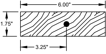
⑥ TOP RAIL - GLAZED SIDELITE WOOD (0.44 MIN. S.G.)
