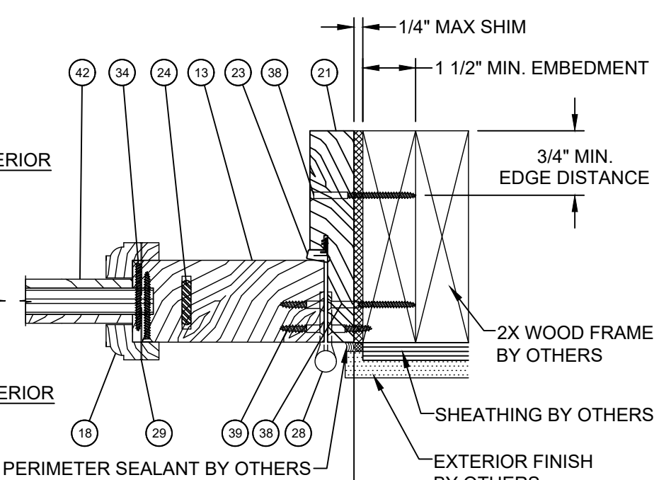
R HORIZONTAL SECTION WOOD FRAME SUBSTRATE OPAQUE HINGE JAMB
