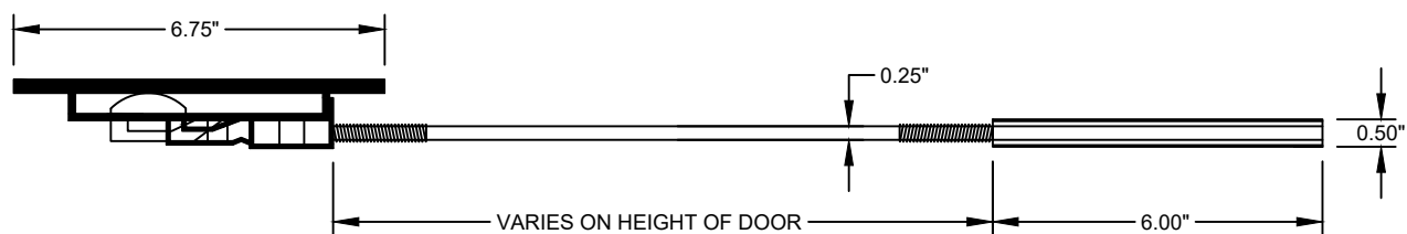
㉗ DELTANA 18EFB EXTENSION FLUSH BOLT OR IVE'S 458 EXTENSION FLUSHBOLT STEEL
