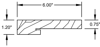
⑥ TOP RAIL - GLAZED SIDELITE WOOD (0.44 MIN. S.G.)
