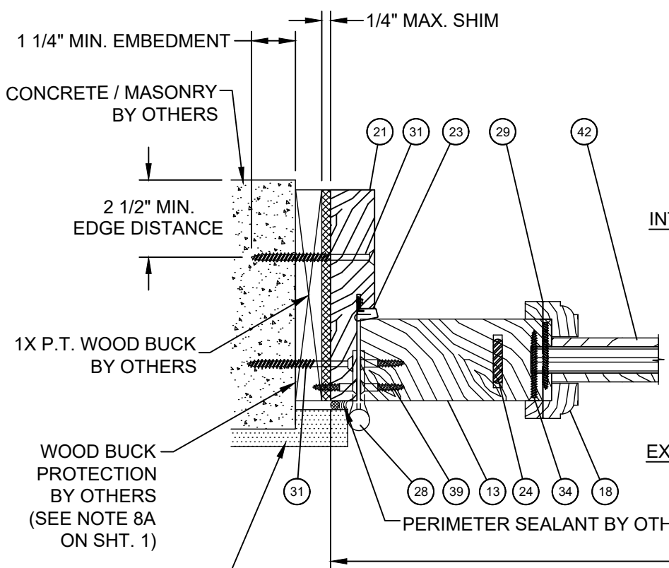
P HORIZONTAL SECTION CONCRETE / MASONRY SUBSTRATE OPAQUE HINGE JAMB
