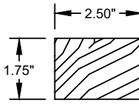
⑩ STILE - GLAZED SIDELITE WOOD (0.44 MIN. S.G.)
