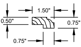
㉓ GLAZING BEAD - GLAZED DOOR WOOD (0.44 MIN. S.G.)
