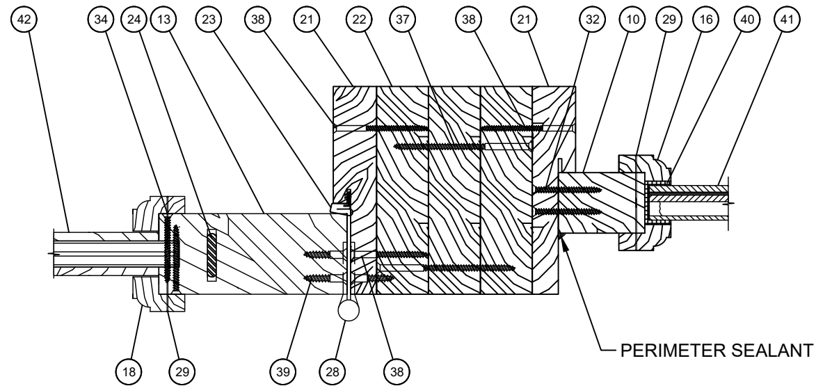
X HORIZONTAL SECTION MULLION OPAQUE DOOR PANEL / GLAZED SIDELITE
