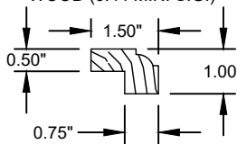
㉔ PANEL STOP - OPAQUE SIDELITE WOOD (0.44 MIN. S.G.)
