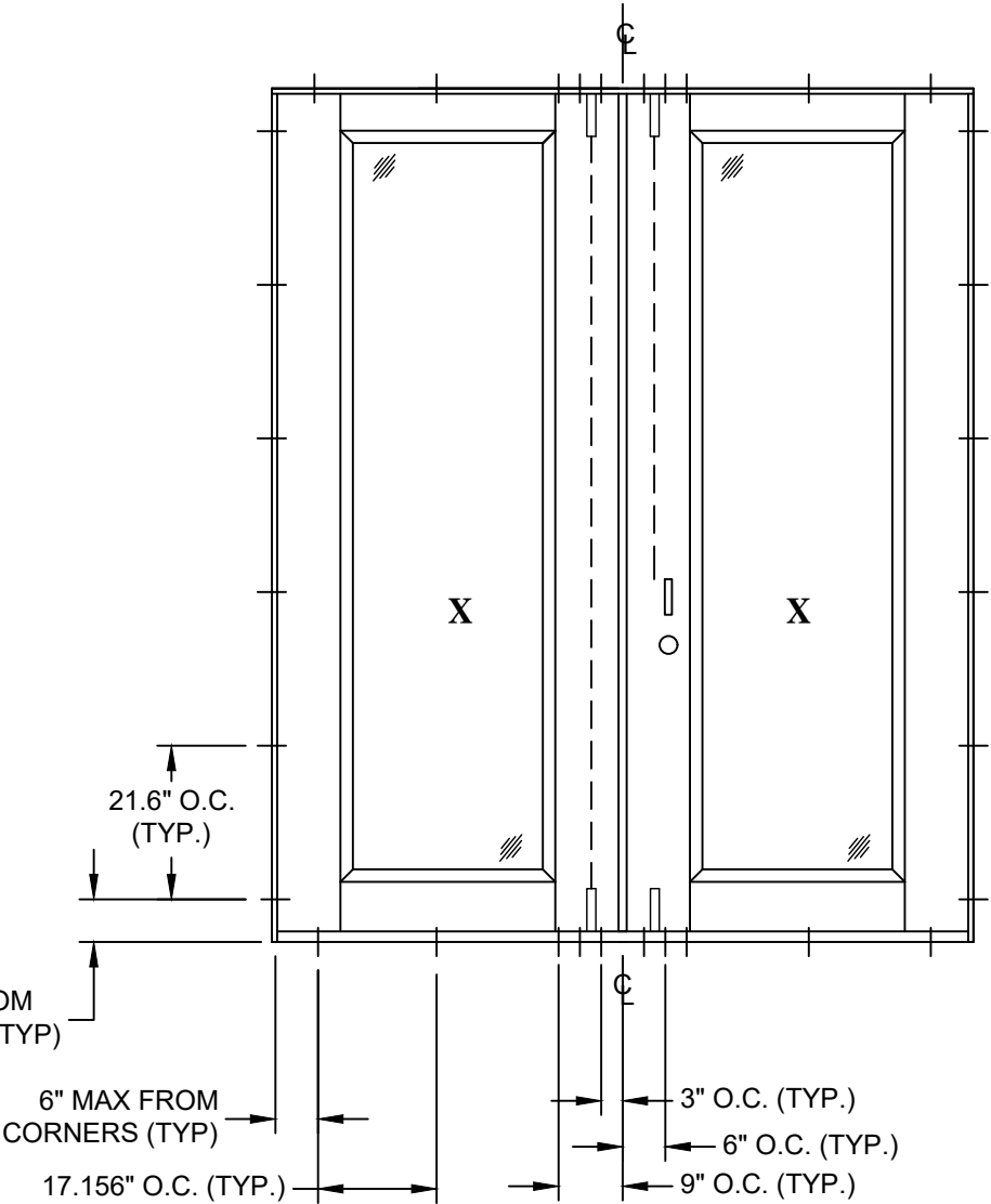
ANCHOR LAYOUT DOUBLE DOOR (XX) SQUARE TOP EXTERIOR VIEW
